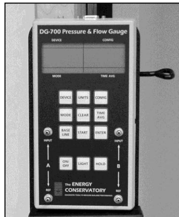
DG-700 Pressure Gauge
