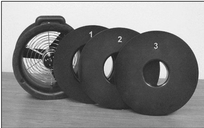
Duct Blaster Fan with 3 Standard Flow Rings
