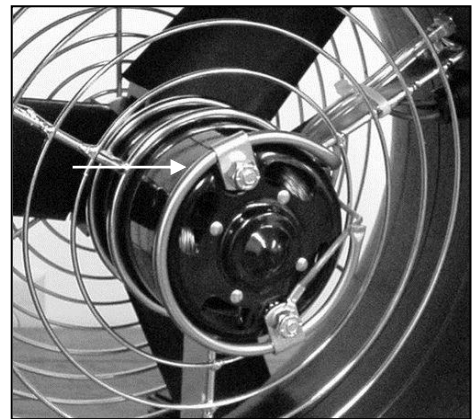
Flow Sensor on Duct Blaster Fan
