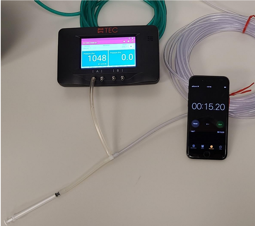
This sensor measures 1048 Pa after 15 seconds. It passes the leak test.
