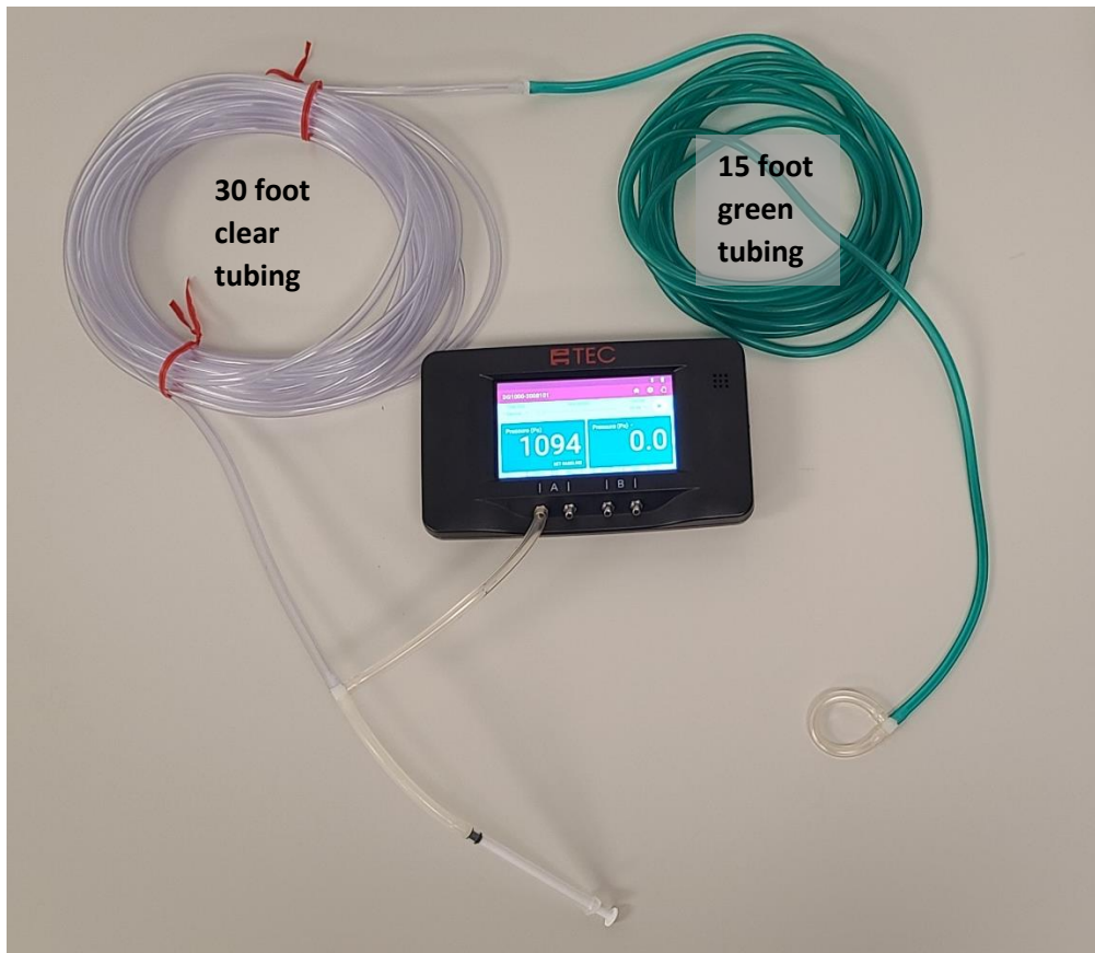
Setup for testing the syringe, tubing, and manometer for leaks.
